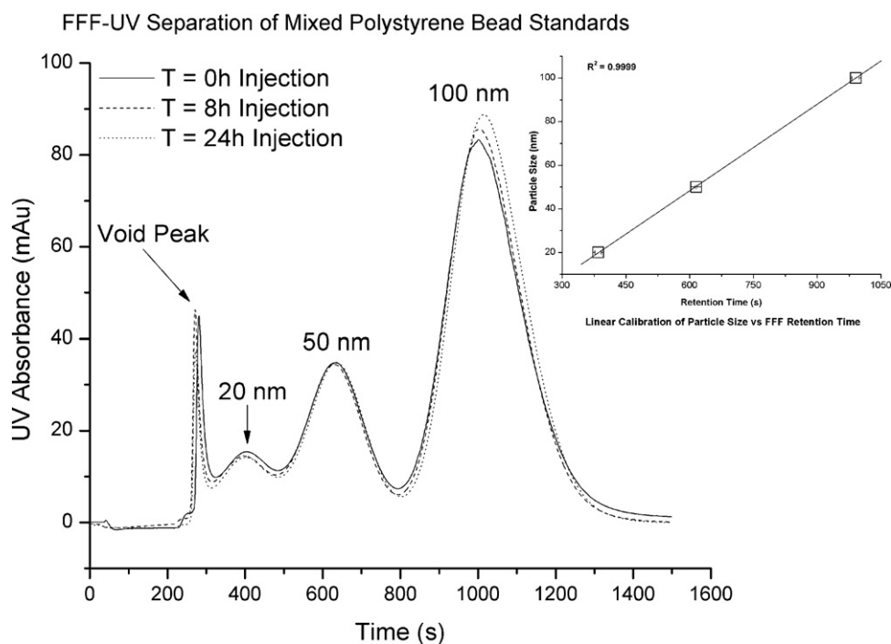
Fig. 1. Overlay of triplicate FFF-UV fractograms of polystyrene bead calibration standards. FFF separation conditions were 1.0 mL/min channel flow and 0.75 mL/min cross flow. UV absorbance detection is at 254 nm wavelength. Inset: Linear regression calibration function using 20, 50, and 100 nm polystyrene bead standards. Error bars represent standard deviation of the triplicate retention times obtained from UV absorbance data at maximum absorbance.
